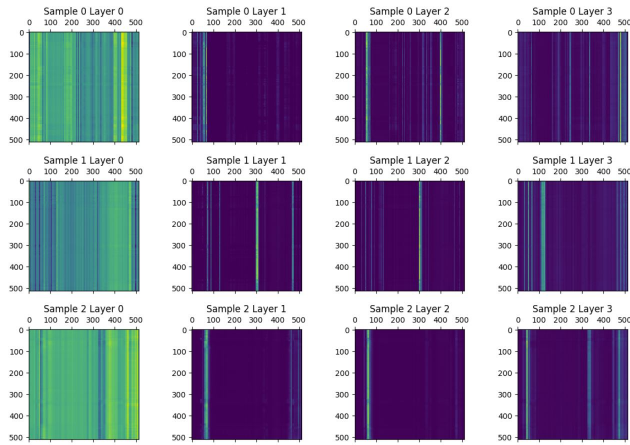
Figure 2: Attention Map of the 4 MHSA Layers for 3 different datapoints from validation data, All Heads Summed, Y Axis represents Query and X axis represent Key. Sample 0 and sample 2 are pre maintenance and sample 1 is post maintenance. Bright sections indicate high attention.
